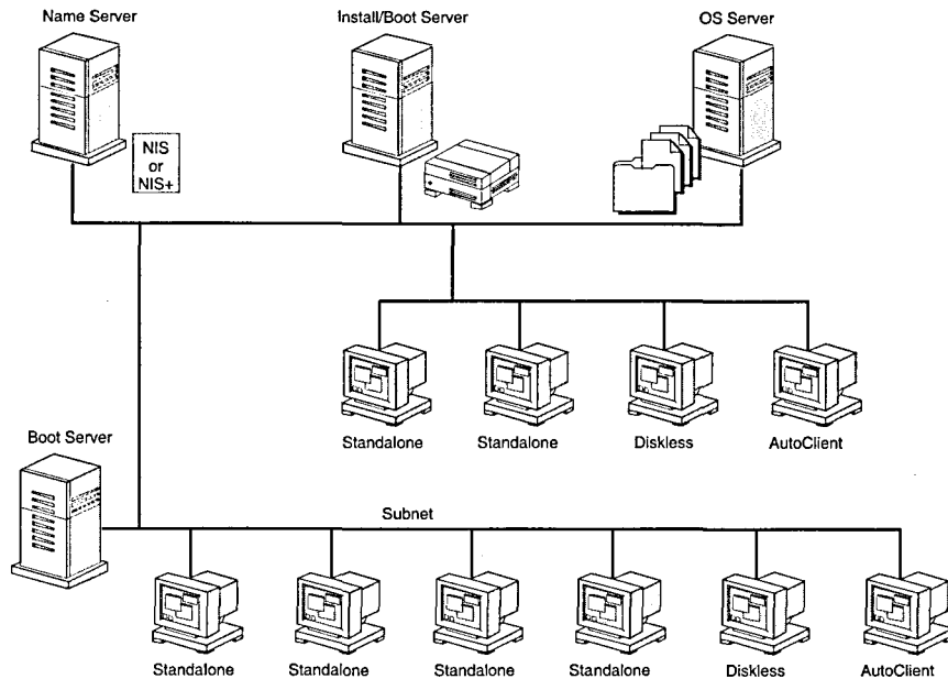
Figure 7-1 Network Installation Servers
